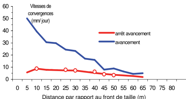
Figure 5 - Vitesses de convergences
