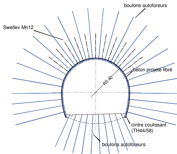
Figure 3 - Profil type 1
